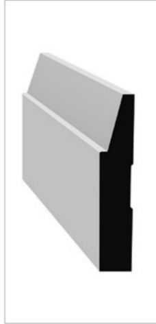
T-114 5/8" x 2-3/4"
